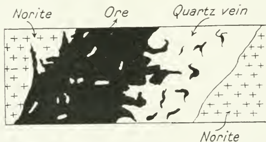
Fig. 34—Diagrammatic sketch showing quartz vein on foot-wall of main ore body, Garson mine, Sudbury area, Ontario. The width of the cross-section represented in the sketch is 20 feet.
